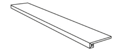
Gradone square assembled 30x120x3,3 . 12"x48"x1 5/16" RETT
